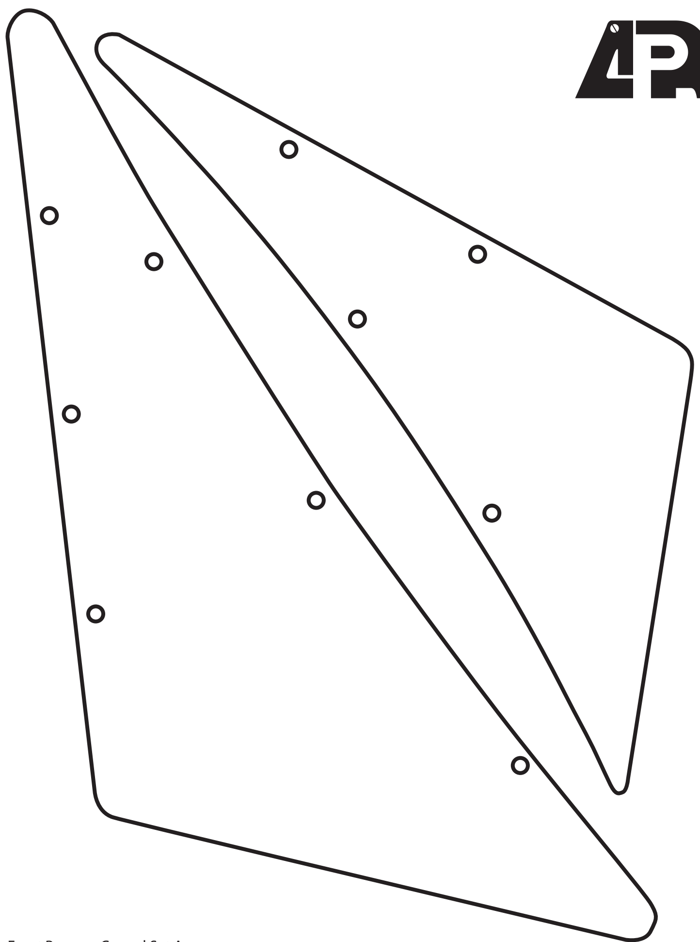
Front Bumper Canard Set A Part Num. #AB-200300
